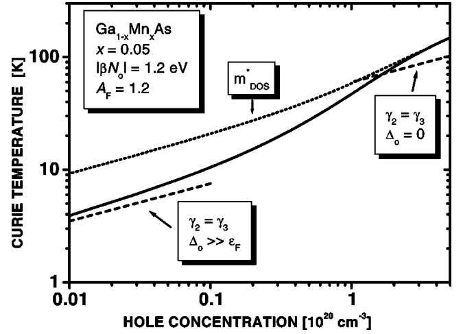
FIG. 4. Curie temperature as a function of the hole concentration for \text{Ga}_{0.95}\text{Mn}_{0.05}\text{As} computed from the 6 \times 6 Luttinger model (solid line). Straight dashed lines represent results obtained assuming a large and a small value of the spin-orbit splitting \Delta_0 , respectively. The dotted line is calculated neglecting the effect of the spin-orbit interaction on the hole spin susceptibility.
